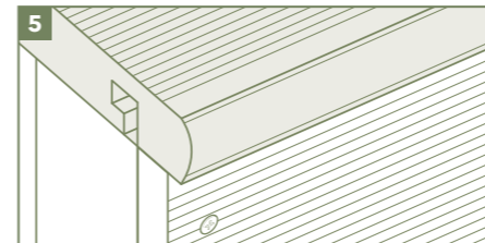
5 STARTER BOARDS: Used to complete the front edge of your deck.
