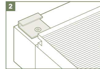
2 STARTER CLIPS: Fitted to the intersection of each joist.
